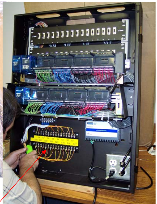
The customer was able to reclaim valuable rack space by moving their controls from a rack mount to a wall mount setup.
