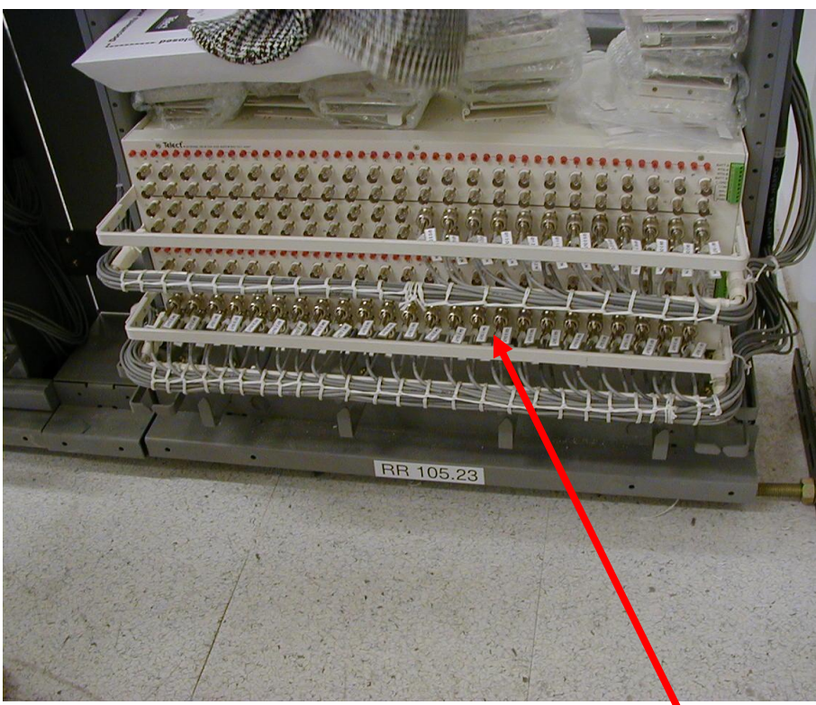
Proper labeling, with optional "flag-tags"
